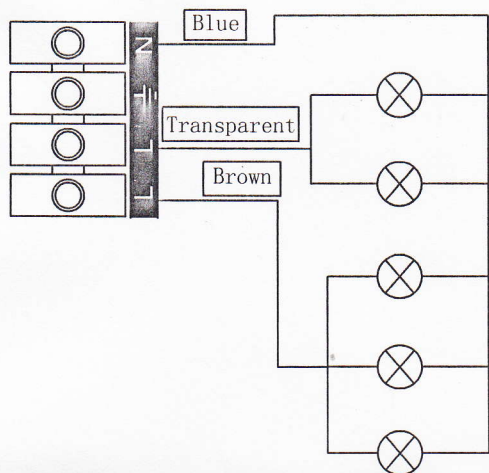
Electrical diagram
